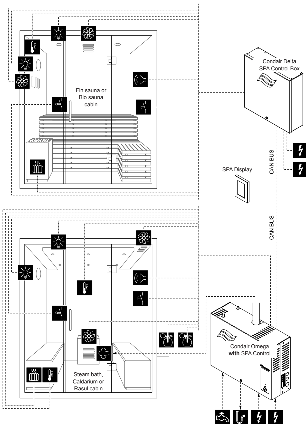
Fig. 9: Condair Delta SPA Control Box and Condair Omega with SPA Control Board for dual cabin applications for medium size cabins
