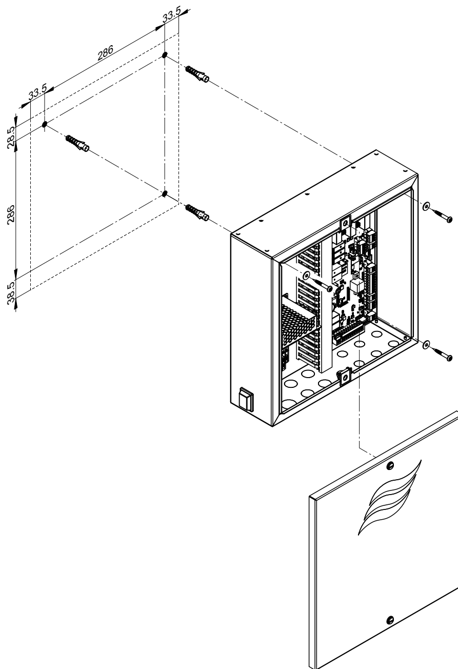
Fig. 11: Mounting the Condair Delta SPA Control Box
